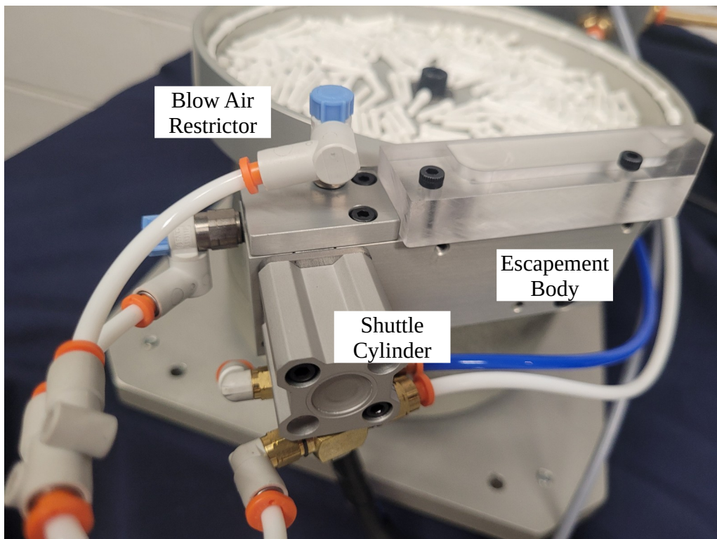
Figure 4: Parts Escapement
